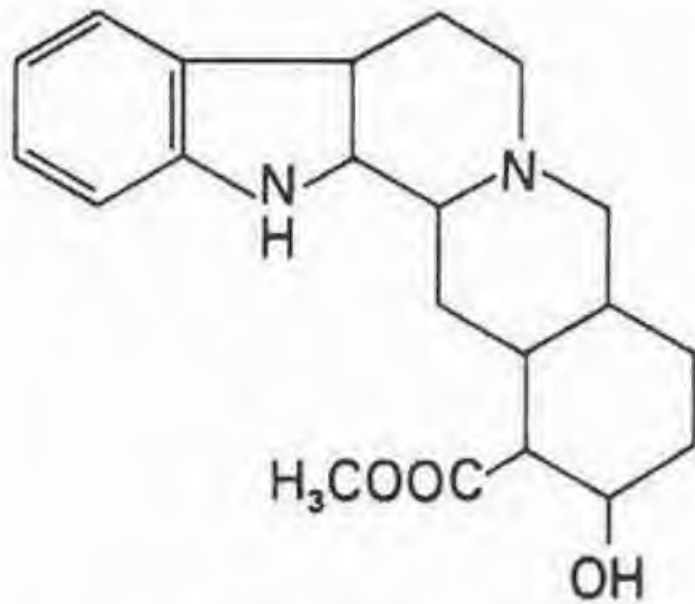
YOHIMBINE
